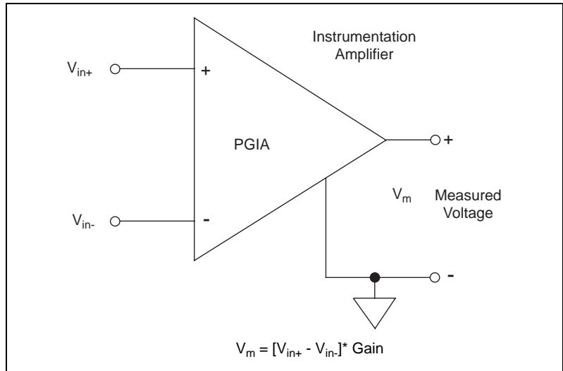
Figure 4-4. DAQPad-6070E PGIA
