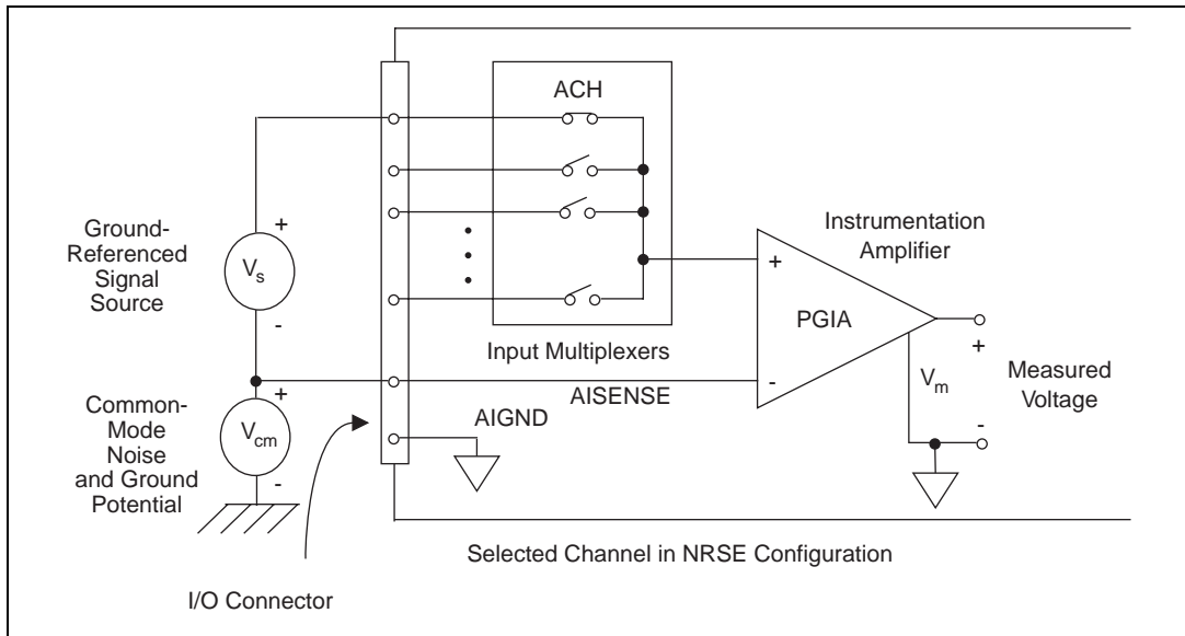
Figure 4-9. Single-Ended Input Connections for Ground-Referenced Signals
