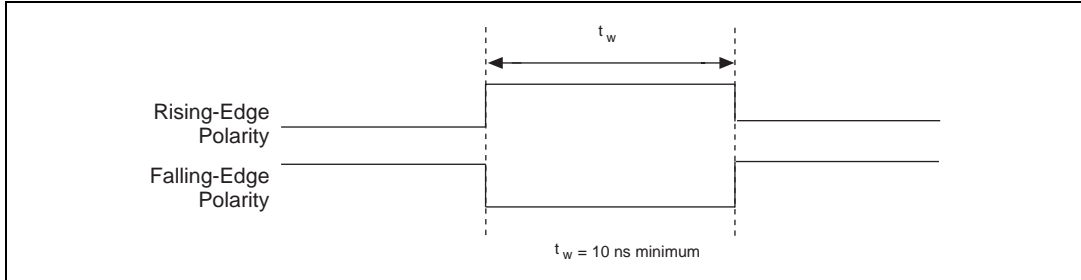
Figure 4-32. GPCTR0_GATE Signal Timing in Edge-Detection Mode
