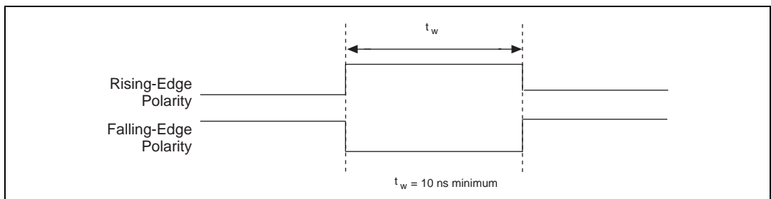
Figure 4-17. TRIG1 Input Signal Timing
