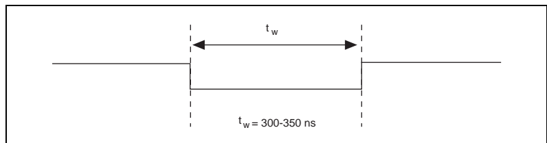
Figure 4-29. UPDATE* Output Signal Timing
