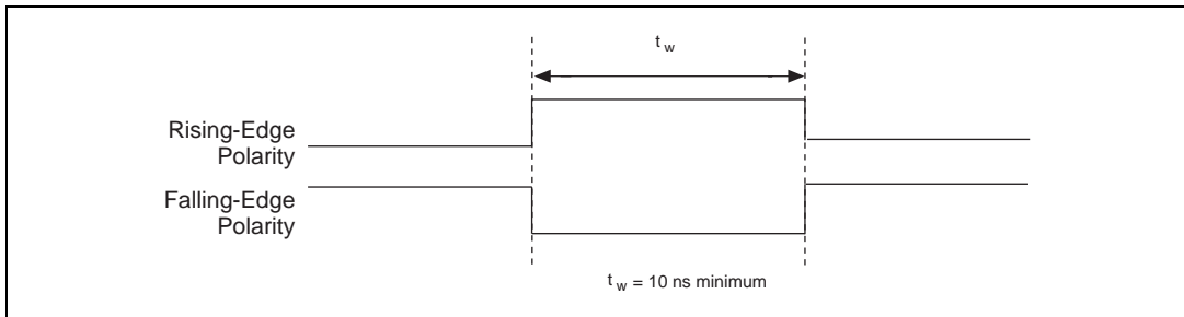
Figure 4-26. WFTRIG Input Signal Timing
