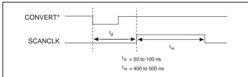
Figure 4-15. SCANCLK Signal Timing
