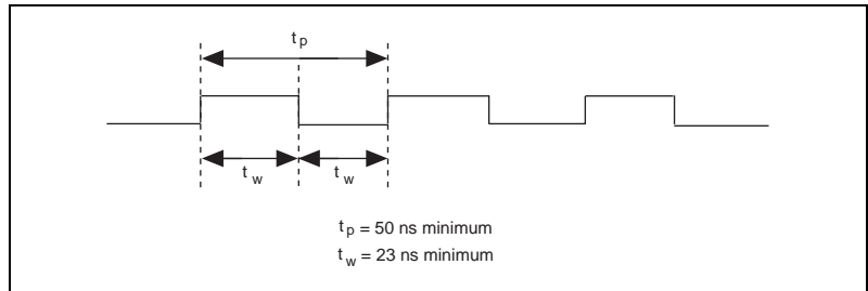
Figure 4-31. GPCTR0_SOURCE Signal Timing
