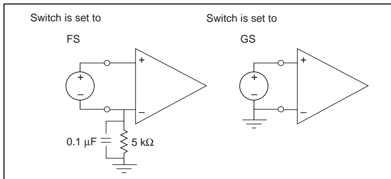
Figure 4-1. Floating Source and Grounded Source Connections
