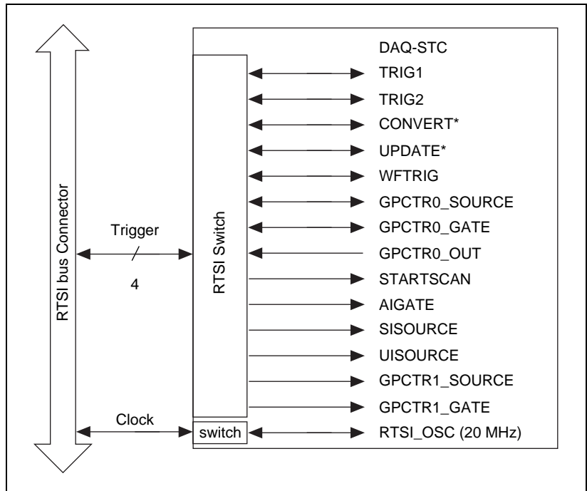
Figure 3-10. RTSI Bus Signal Connection
