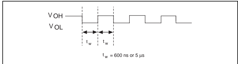
Figure 4-16. EXTSTROBE* Signal Timing
