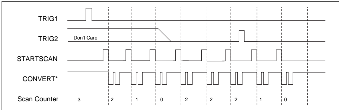
Figure 4-14. Typical Pretriggered Acquisition
