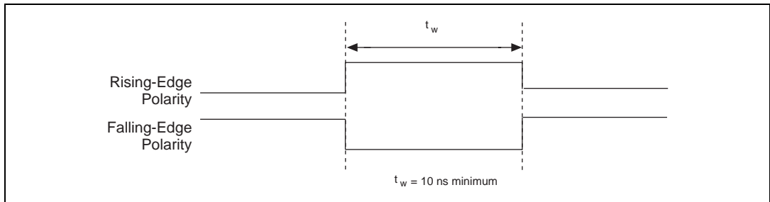
Figure 4-19. TRIG2 Input Signal Timing
