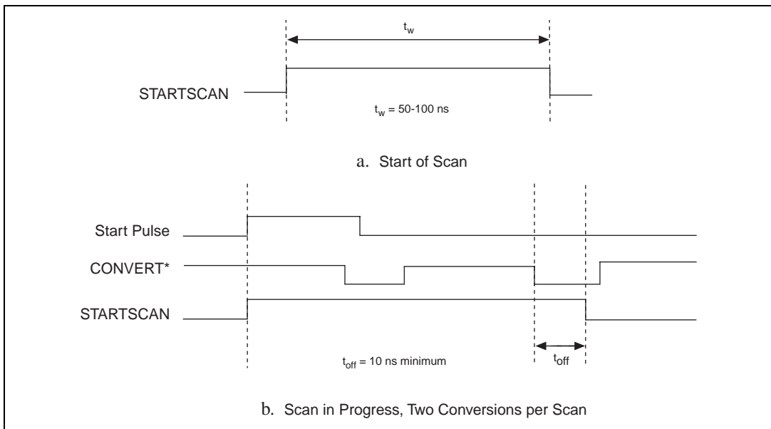
Figure 4-22. STARTSCAN Output Signal Timing
