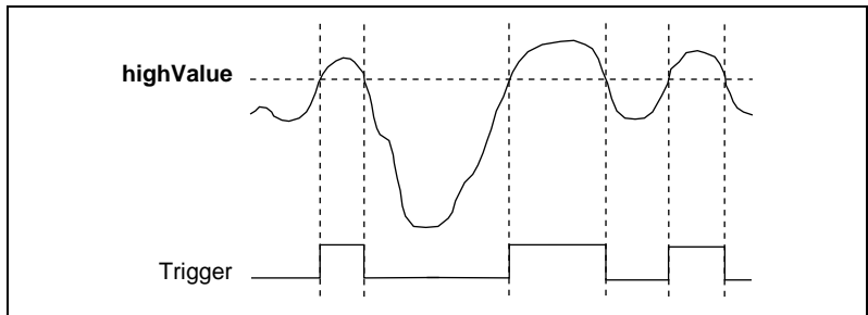
Figure 3-5. Above-High-Level Analog Triggering Mode
