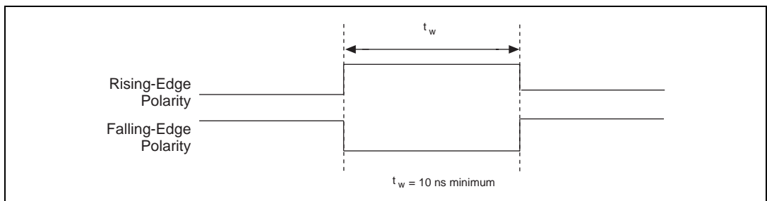
Figure 4-23. CONVERT* Input Signal Timing
