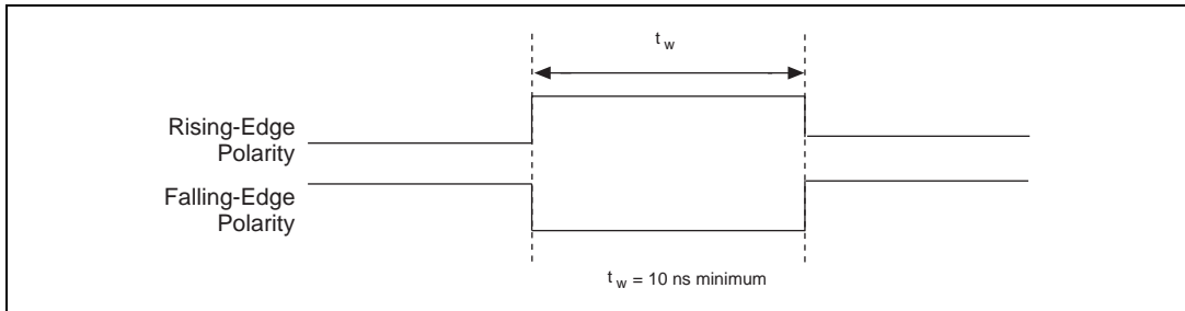
Figure 4-21. STARTSCAN Input Signal Timing
