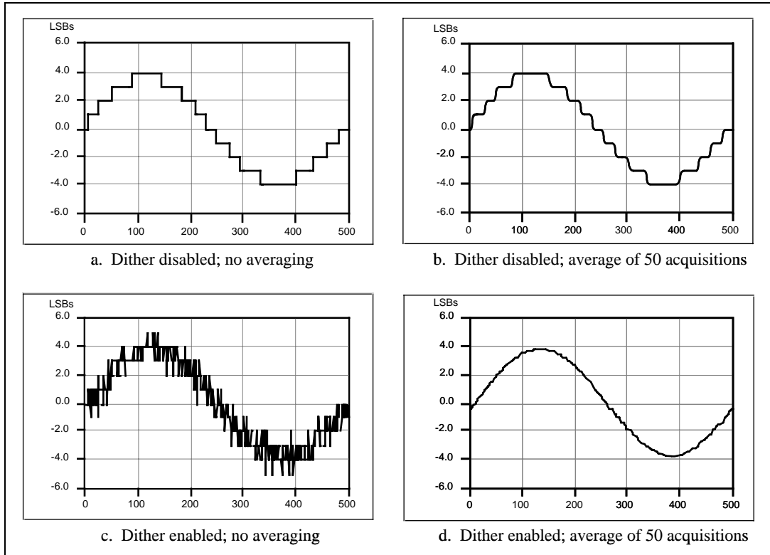
Figure 3-2. Dither
