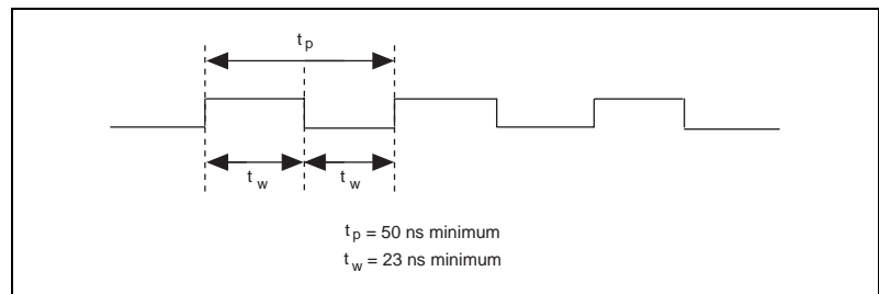
Figure 4-34. GPCTR1_SOURCE Signal Timing
