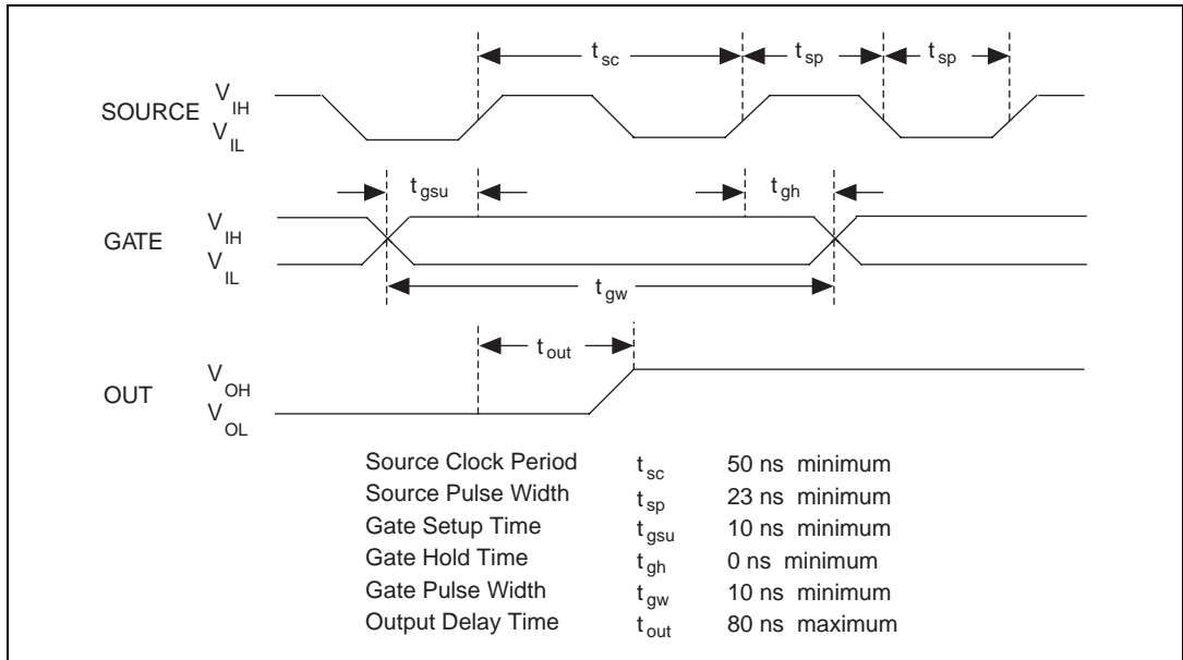
Figure 4-37. GPCTR Timing Summary
