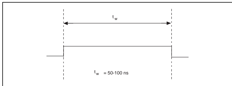
Figure 4-27. WFTRIG Output Signal Timing
