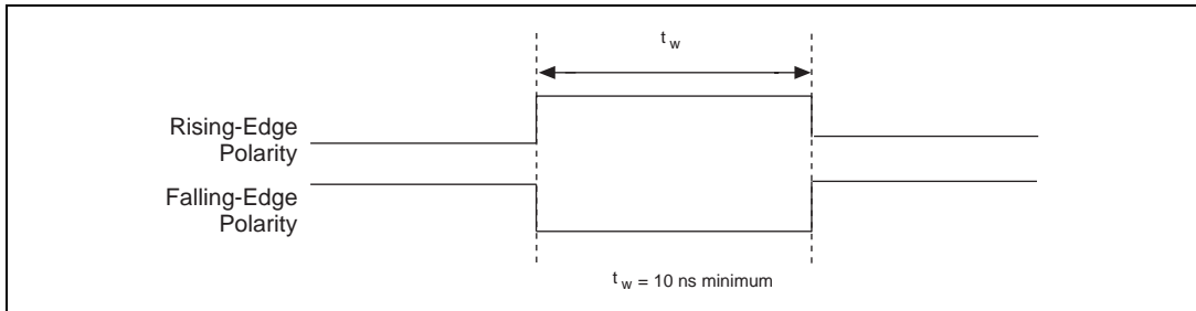
Figure 4-35. GPCTR1_GATE Signal Timing in Edge-Detection Mode
