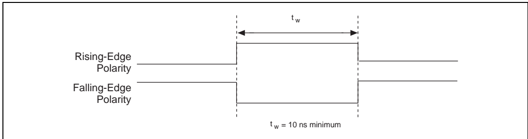
Figure 4-28. UPDATE* Input Signal Timing
