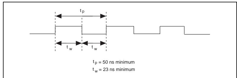
Figure 4-25. SISOURCE Signal Timing
